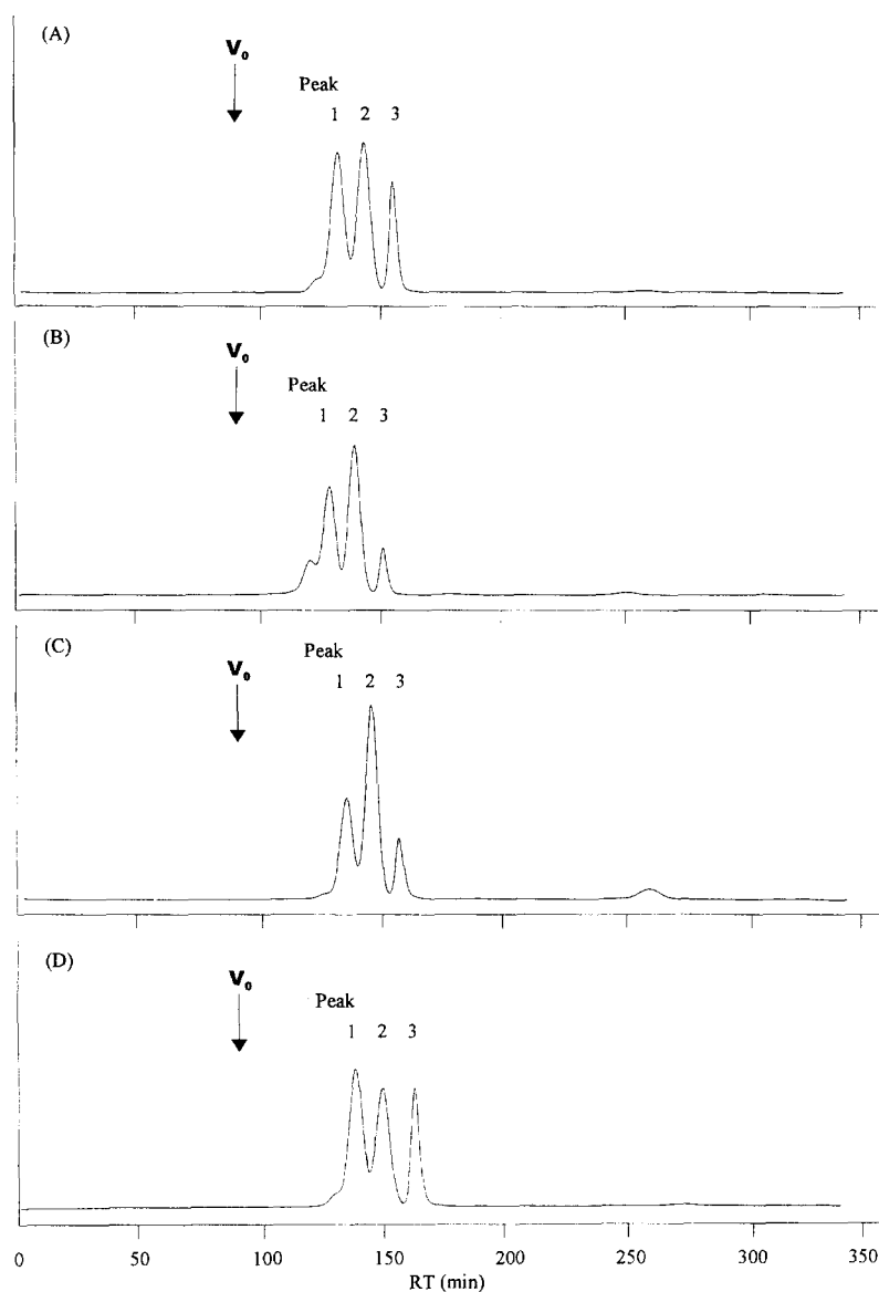
Fig. 4. Elution profiles of the reaction products from Alg-Na (A), polyM (B), polyG (C) and MG random (D) blocks generated by the Alteromonas alginate lyase. Substrate solutions containing 6 to 7 mg/mL of each in 0.1 M Tris-HCl buffer (pH 7.5) were incubated for 12 h at 30 °C with the 150 U/mL purified alginate lyase of Alteromonas sp. H-4. The reaction mixture was applied to a column (1.34 cm \times 40 cm) of Cellulofine GCL25m (Seikagaku Corporation) and eluted with 0.1 M \text{Na}_2\text{SO}_4 at 25 mL/h. The reaction products from substrate depolymerization were detected at 235 nm using a Hitachi L-4200 UV-VIS detector. The arrow indicates the void volume of the column.
