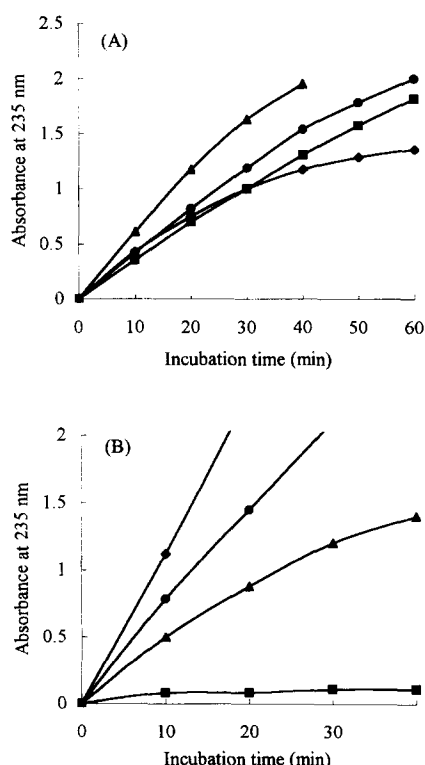
Fig. 2. Substrate specificity of the purified extracellular alginate lyase of Alteromonas sp. strain H-4 (A) and abalone alginate lyase (B). Alginate lyase activity at 30 °C was measured for the following substrates; sodium alginate (●), polyM block (◆), polyG block (■) and MG random block (▲) by monitoring the absorbance of reaction mixture at 235 nm.
