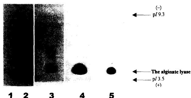
Fig. 3. Activity staining profiles of the extracellular alginate lyase of Alteromonas sp. H-4 for polyM block and polyG block after isoelectric focusing gel electrophoresis. Lane 1, marker proteins (see Fig. 2, panel C); lane 2, the alginate lyase (0.15 \mu g) stained with CBB R250; lane 3, activity staining with gel-overlay containing Alg-Na; lane 4, activity staining with gel overlay containing polyM; lane 5, activity staining with gel overlay containing polyG.
