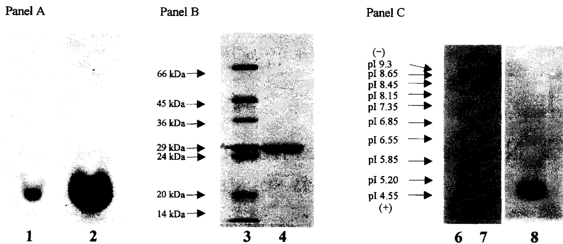
Fig. 1. Homogeneity of the purified extracellular alginate lyase of Alteromonas sp. H-4. (Panel A) Native-PAGE (7% gel) of the purified alginate degrading enzyme. Lane 1, the alginate lyase (3.4 \mu g) stained with CBB R250; lane 2, activity staining with gel-overlay containing alginate. (Panel B) SDS-PAGE (10% gel) of the purified enzyme. Lane 3, markers [albumin (bovine): 66 kDa, ovalbumin: 45 kDa, glyceraldehyde-3-phosphate dehydrogenase: 36 kDa, carbonic anhydrase: 29 kDa, trypsinogen: 24 kDa, trypsin inhibitor: 20.1 kDa, \alpha -lactalbumin: 14.2 kDa]; lane 4, the alginate lyase (30 \mu g) stained with CBB R250. (Panel C) Isoelectric focusing of the enzyme. Lane 6, marker proteins [trypsinogen: pI 9.30, lentil lectin-basic band: pI 8.65, lentil lectin-middle band: pI 8.45, lentil lectin-acidic band: pI 8.15, horse myoglobin-basic band: pI 7.35, horse myoglobin-acidic band: pI 6.85, human carbonic anhydrase B: pI 6.55, bovine carbonic anhydrase B: pI 5.85, \beta -lactoglobulin A: pI 5.20, soybean trypsin inhibitor pI 4.55]; lane 7, the alginate lyase (0.15 \mu g) stained with CBB R250; lane 8, activity staining with gel-overlay containing alginate.
